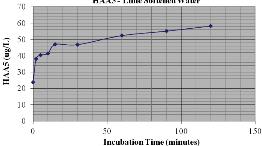
Figure 6 – City of Boca Raton Lime-Softened Water HAA5FP Curve
