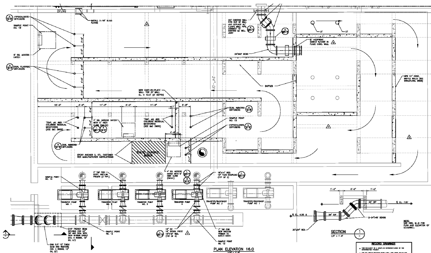
Figure 8. BCWWS WTP 1A East Clearwell
